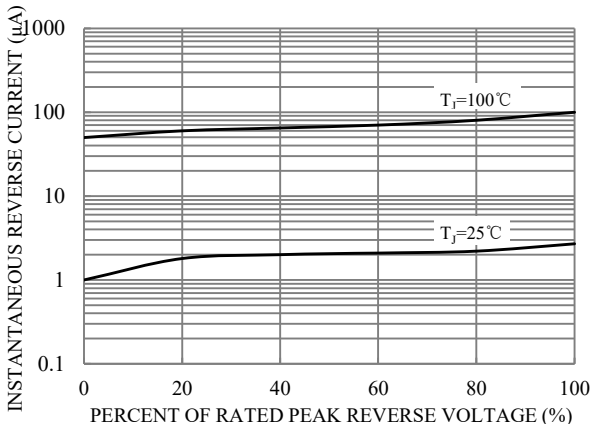
Fig.3-TYPICAL REVERSE CHARACTERISTICS
