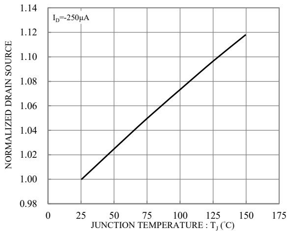
Fig.11 Drain Source Breakdown Voltage vs. Junction Temperature
