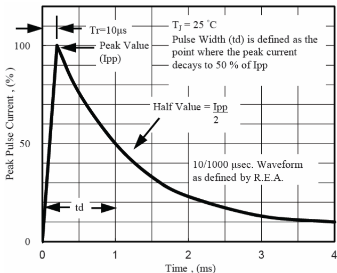
Fig. 5 - Pulse Waveform
