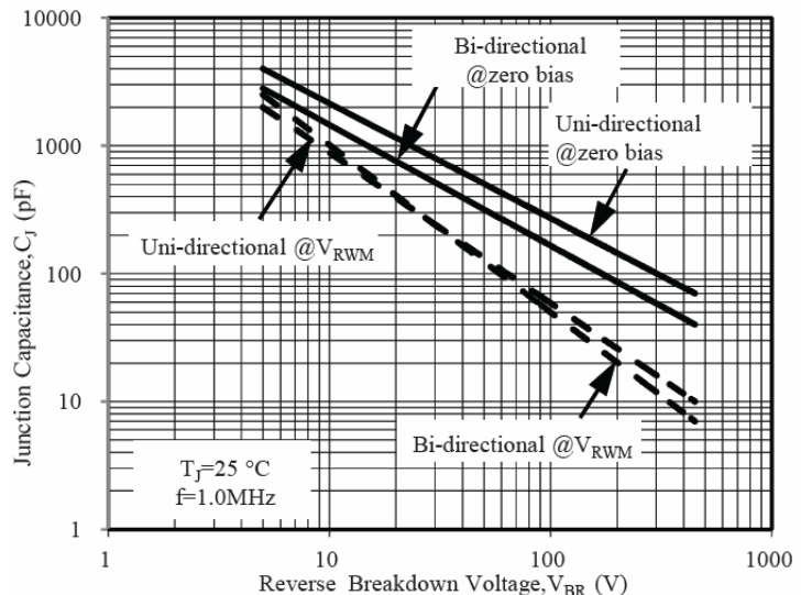
Fig. 6 - Typical Junction Capacitance
