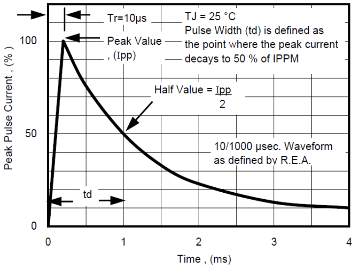
Fig. 5 - Pulse Waveform
