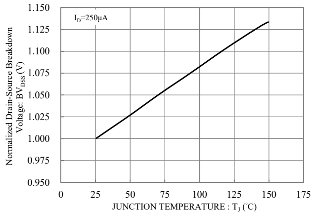
Fig.10 Brekdown Voltage vs Junction Temperature
