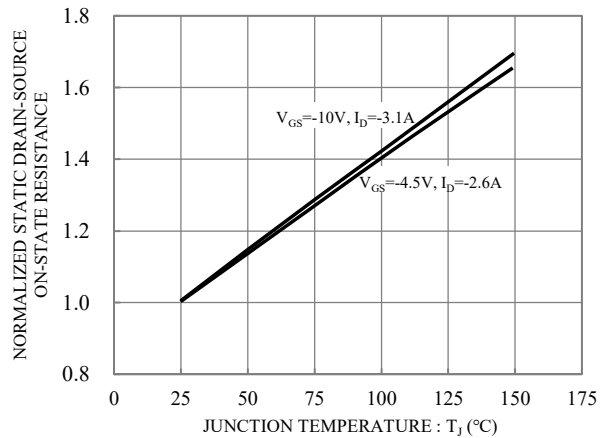
Fig.6 Normalized Static Drain-Source On-state Resistance vs. Junction Temperature
