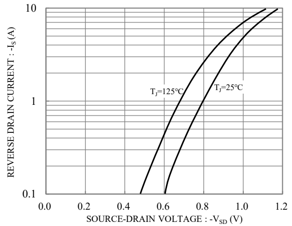
Fig.10 Typical Forward Characteristic
