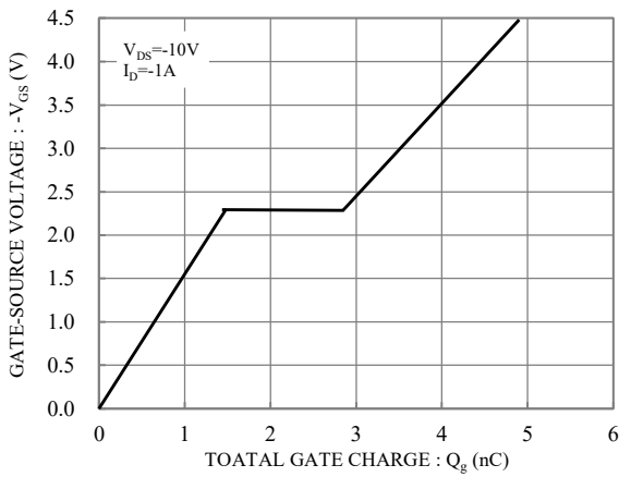
Fig.9 Gate Charge
