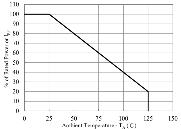
Fig.2-Power Derating Curve
