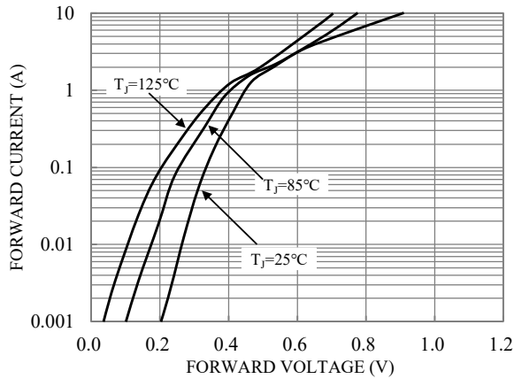
Fig.1-TYPICAL FORWARD CHARACTERISTICS
