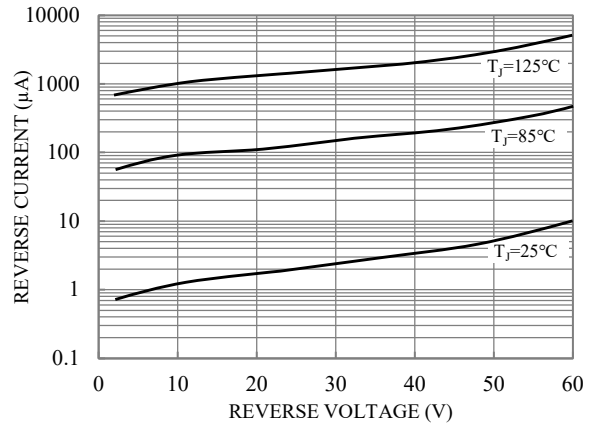
Fig.2-TYPICAL REVERSE CHARACTERISTICS
