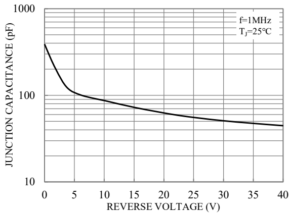
Fig.3-CAPACITANCE
