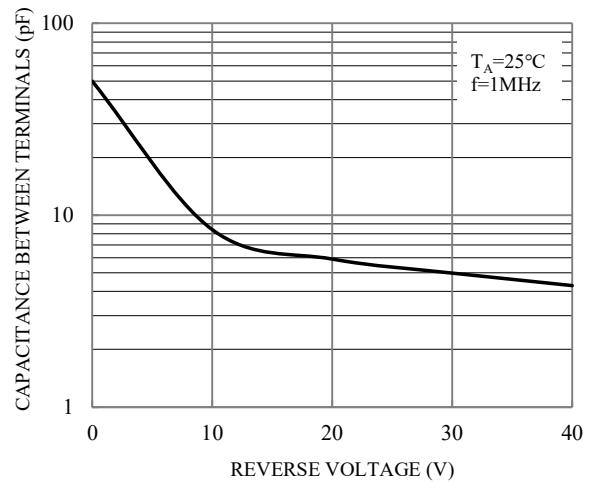
Fig.4-TOTAL CAPACITANCE
