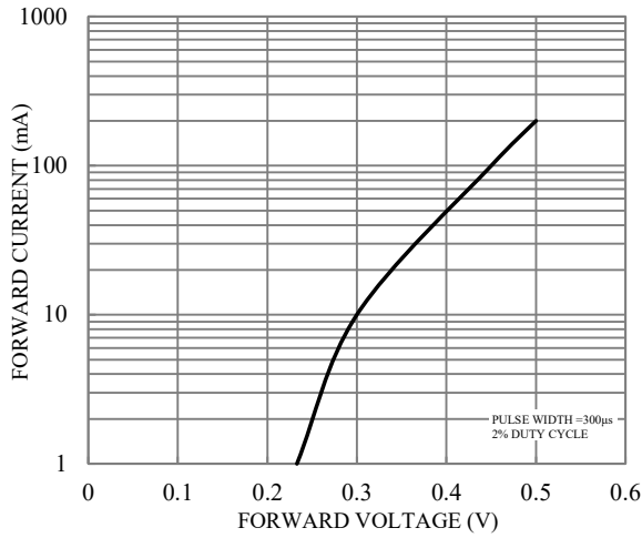
Fig.1-TYPICAL FORWARD CHARACTERISTICS
