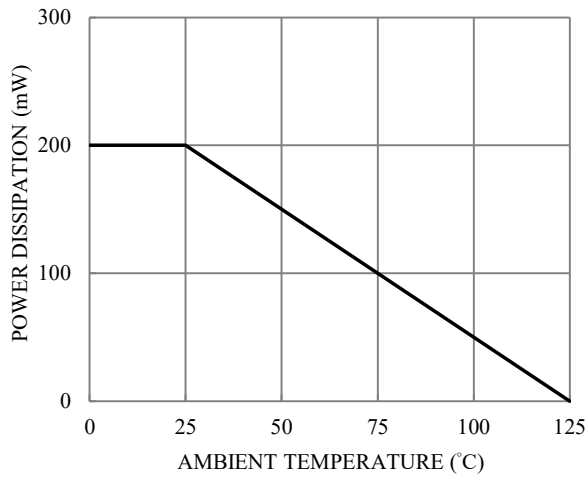
Fig.3-POWER DETATING CURVE
