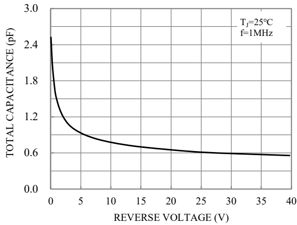
Fig. 3-TYPICAL TOTAL CAPACITANCE
