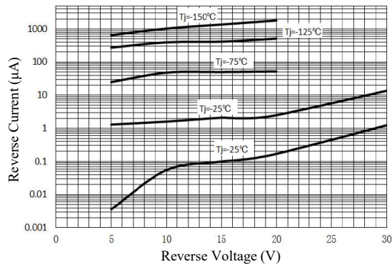
Fig 1. Reverse Characteristics
