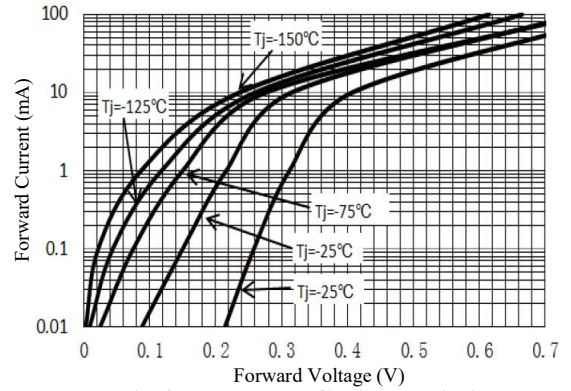
Fig 2. Forward Characteristics
