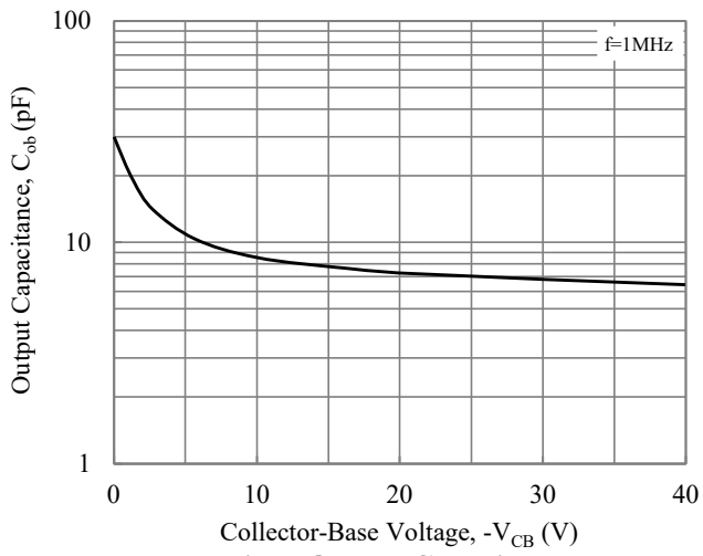
Fig. 7 Output Capacitance
