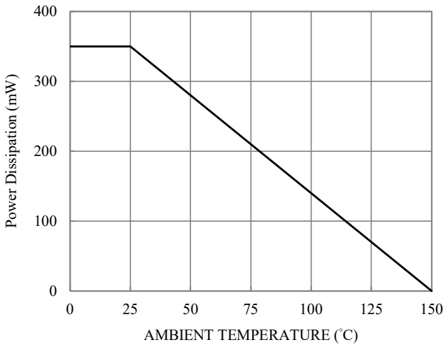
Fig. 1 Power Derating Curves
