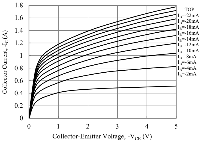
Fig. 5 Output Characteristics
