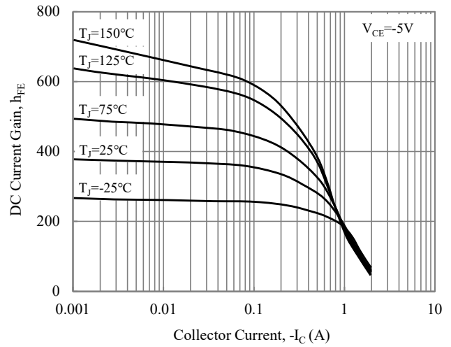
Fig. 2 Current Gain vs. Collector Current
