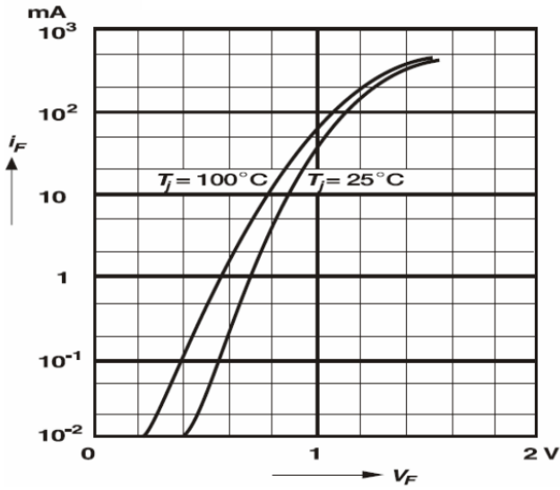
Figure 1. Forward Characteristic
