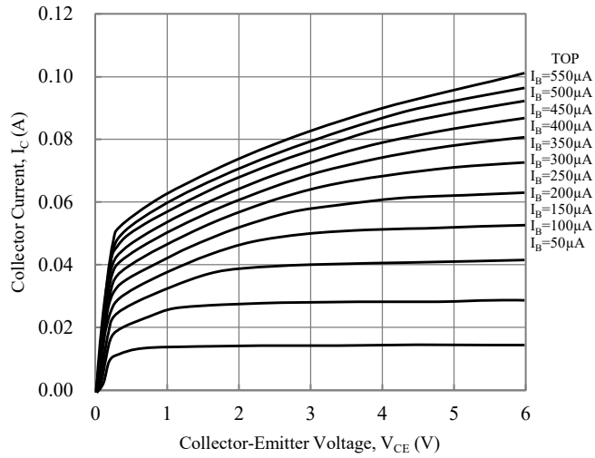
Fig. 7 Output Characteristics Curves
