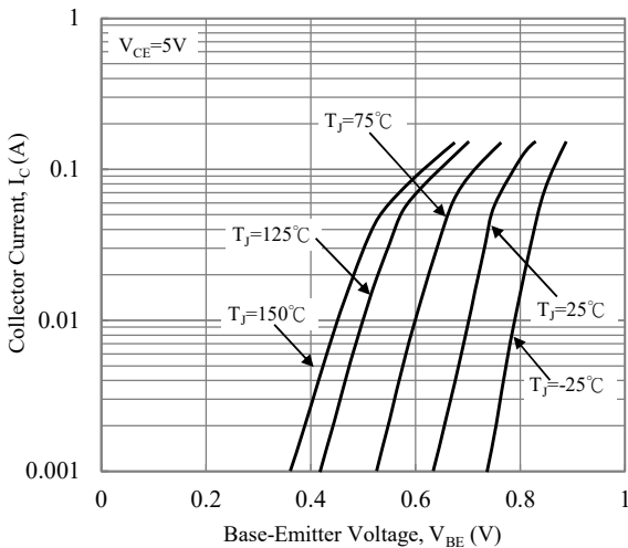
Fig. 5 Base-Emitter Voltage vs. Collector Current
