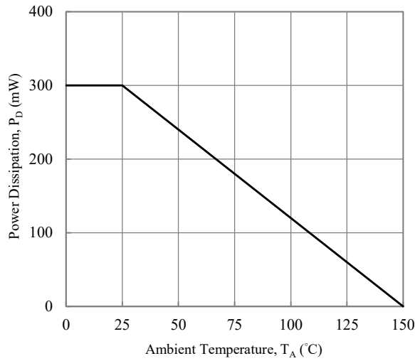
Fig. 1 Power Derating Curves
