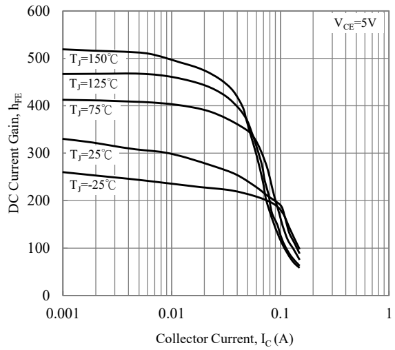
Fig. 2 Current Gain vs. Collector Current
