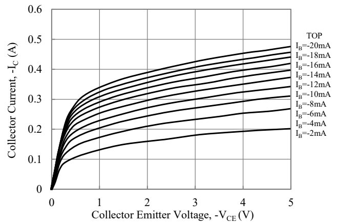
Fig. 12-Output Characteristics Curve
