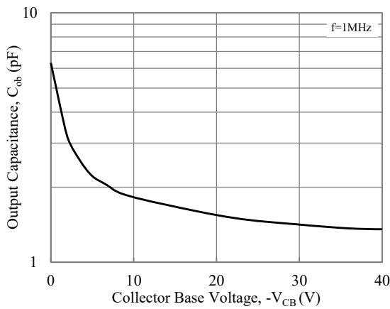
Fig. 11-Output Capacitance
