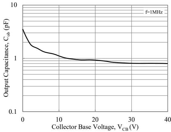
Fig. 5-Output Capacitance
