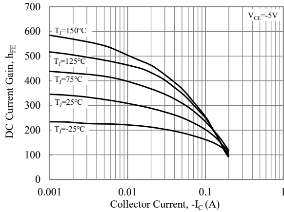
Fig. 7-Current Gain vs. Collector Current
