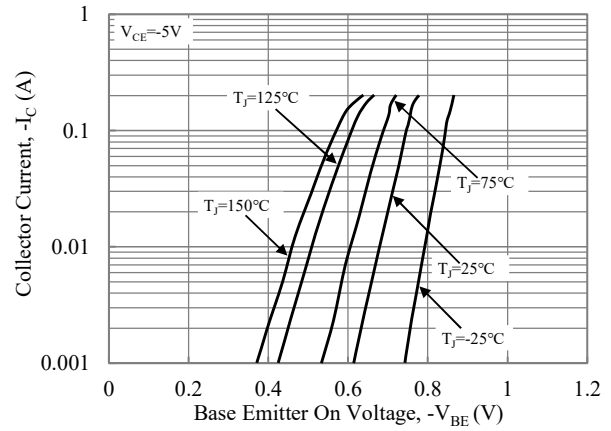
Fig. 10-Base Emitter Voltage vs. Collector Current
