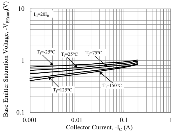
Fig. 9-Base Emitter Saturation Voltage vs. Collector Current
