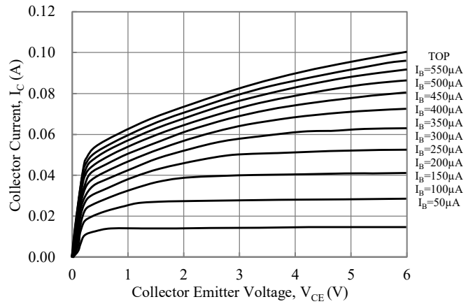
Fig. 6-Output Characteristics Curve
