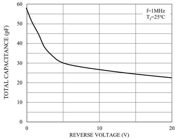
Fig.3-CAPACITANCE
