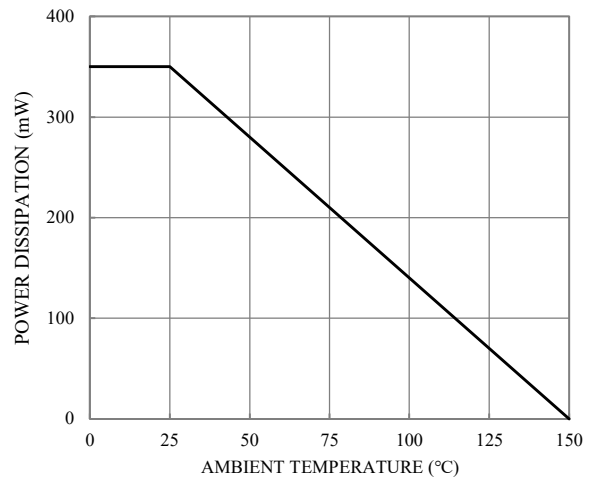
Fig.4-DERATING CURVE
