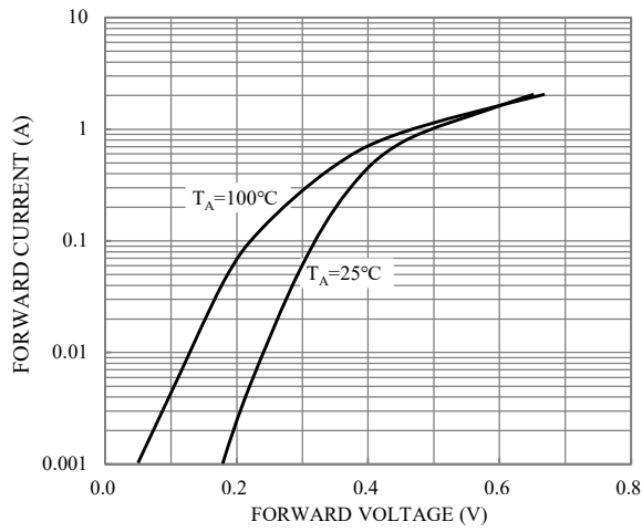
Fig.1-TYPICAL FORWARD CHARACTERISTICS
