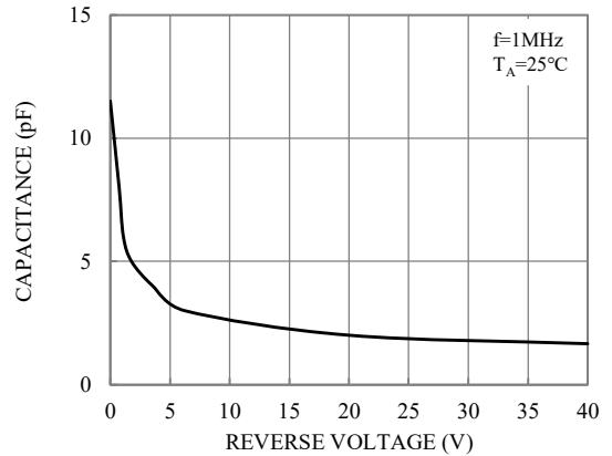
Fig.4-TOTAL CAPACITANCE
