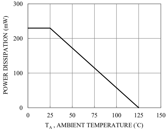
Fig.1-POWER DERATING CURVE
