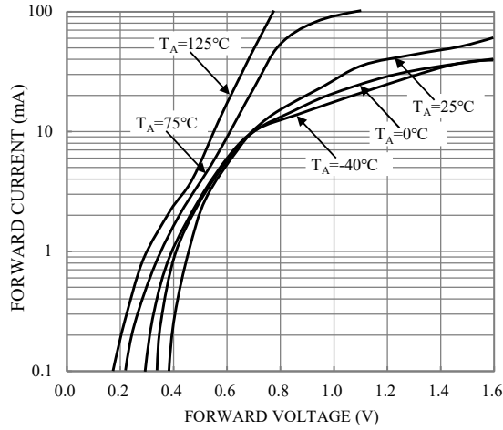
Fig.1-TYPICAL FORWARD CHARACTERISTICS
