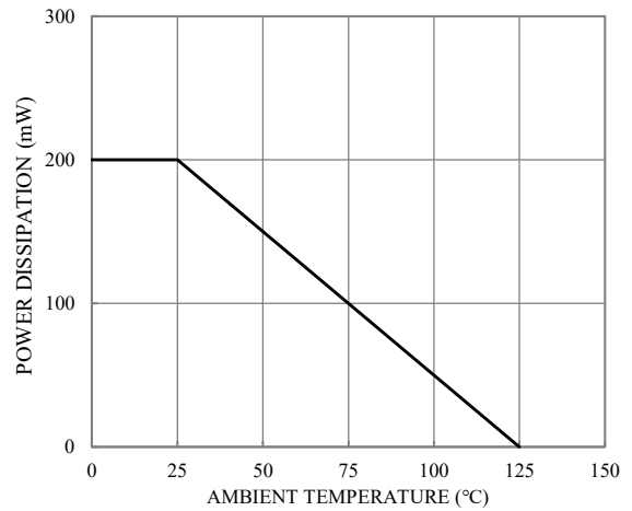
Fig.4-POWER DERATING CURVE
