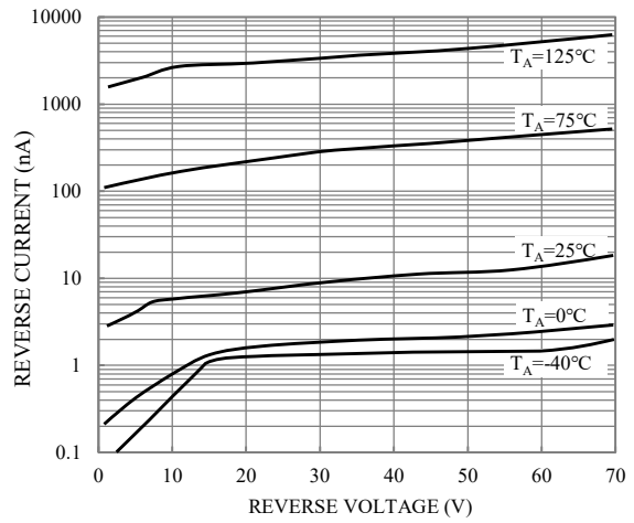
Fig.2-TYPICAL REVERSE CHARACTERISTICS
