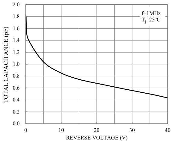
Fig.3-CAPACITANCE
