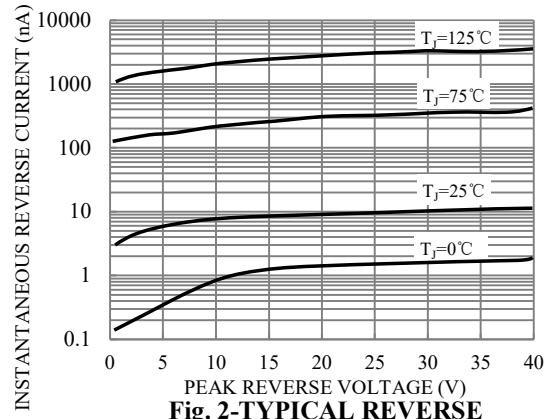
Fig. 2-TYPICAL REVERSE CHARACTERISTICS
