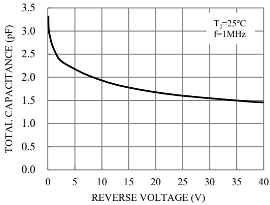
Fig. 3-TYPICAL TOTAL CAPACITANCE
