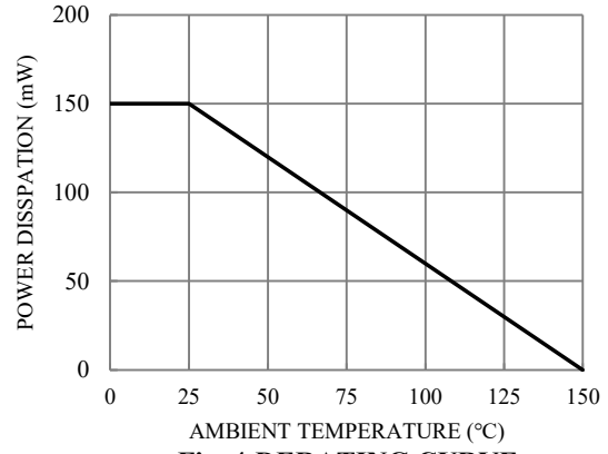
Fig. 4-DERATING CURVE
