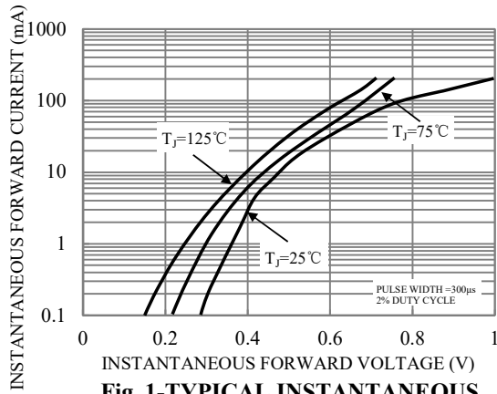
Fig. 1-TYPICAL INSTANTANEOUS FORWARD CHARACTERISTICS
