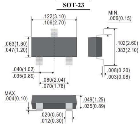
Dimension in inches and (millimeters)
