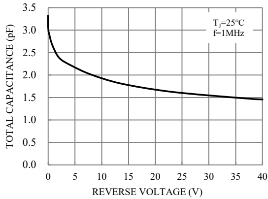
Fig. 3-TYPICAL TOTAL CAPACITANCE
