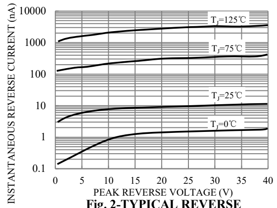
Fig. 2-TYPICAL REVERSE CHARACTERISTICS
