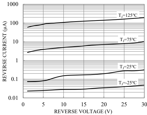
Fig.3-REVERSE CHARACTERISTICS CURVE
