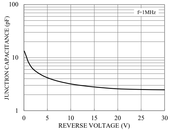
Fig.4-JUNCTION CAPACITANCE
