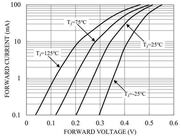
Fig.2-FORWARD CHARACTERISTICS CURVE
