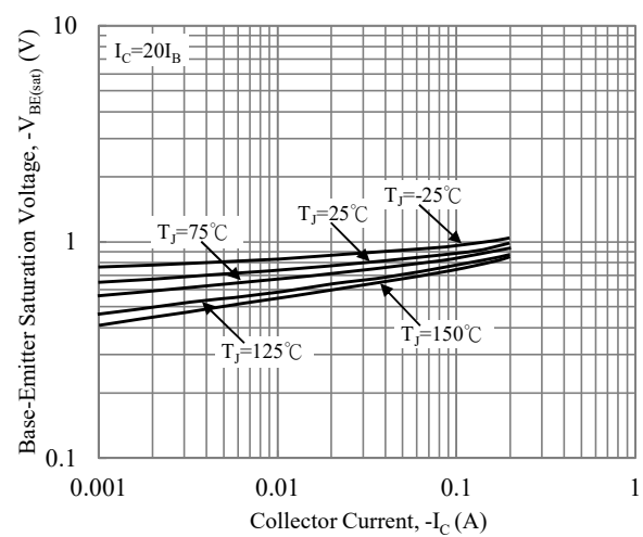
Fig. 4 Base-Emitter Saturation Voltage vs. Collector Current
