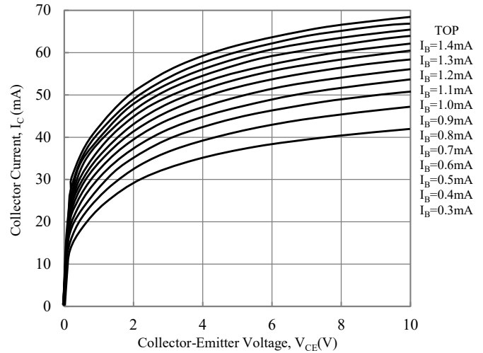
Fig. 2 Collector-Emitter Voltage vs. Collector Current
