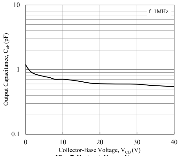
Fig. 7 Output Capacitance
