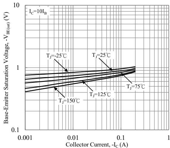
Fig. 5 Base-Emitter Saturation Voltage vs. Collector Current
