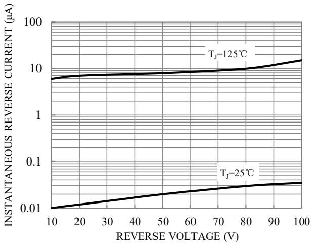
Fig.3-TYPICAL REVERSE CHARACTERISTICS
