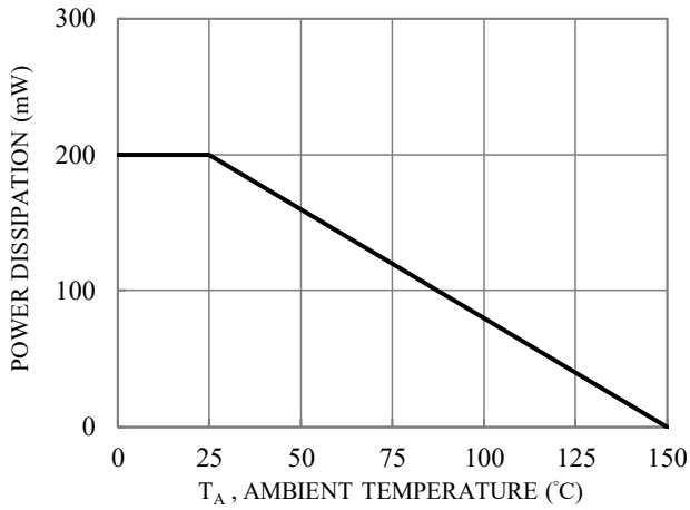
Fig.1-POWER DERATING CURVE
