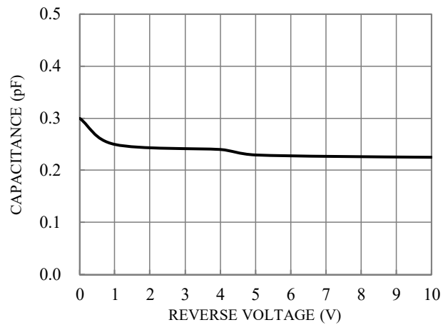
Fig.4- TOTAL CAPACITANCE
