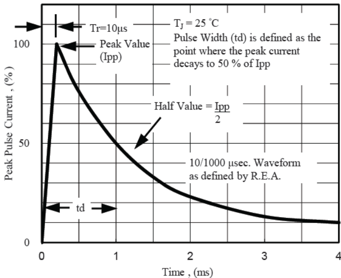
Fig. 5 - Pulse Waveform
