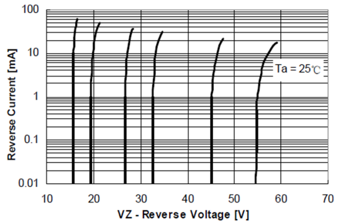
Figure 7. Reverse Current vs. Reverse Voltage
