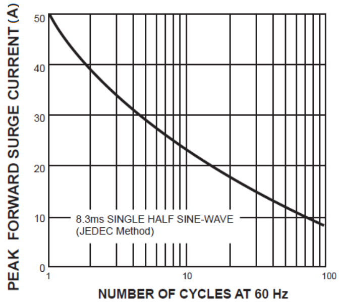
FIG. 2- PEAK FORWARD SURGE CURRENT
