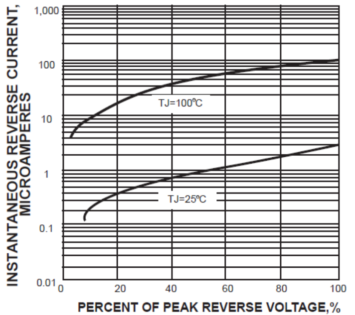
FIG. 4-TYPICAL REVERSE CHARACTERISTICS
