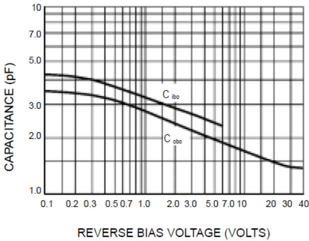
Figure 3. Capacitance
