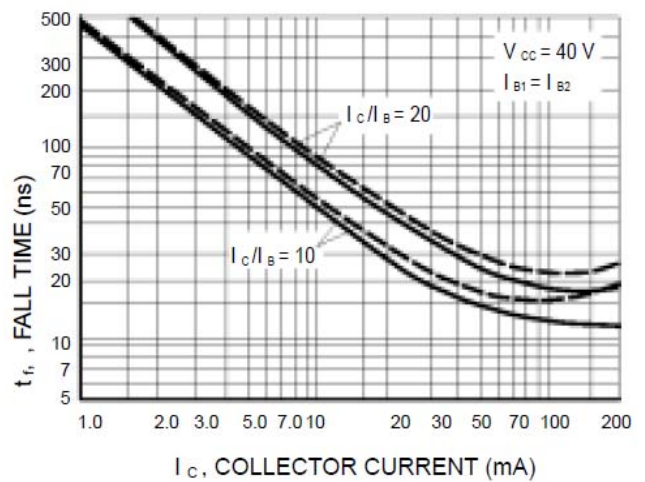
Figure 8. Fall Time
