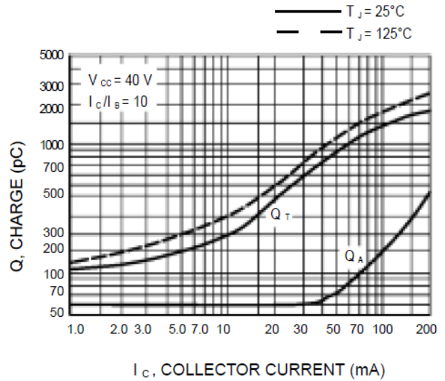
Figure 4. Charge Data
