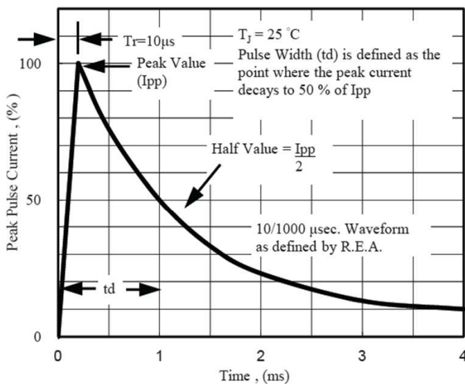
Fig. 5 - Pulse Waveform
