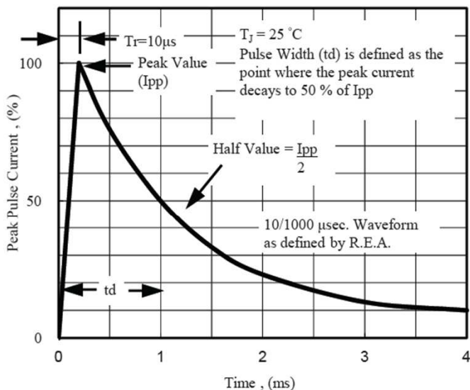
Fig. 5 - Pulse Waveform
