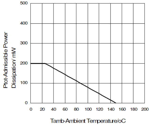
Figure 2. Power De-rating
