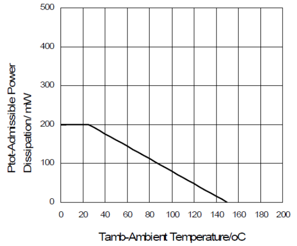
Figure 2. Power De-rating
