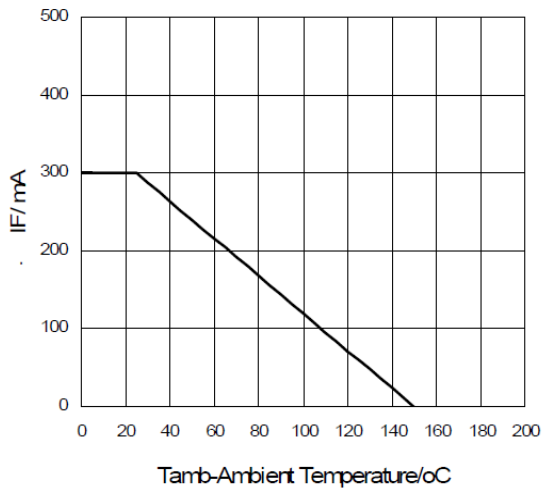
Figure 3. Forward Current De-rating
